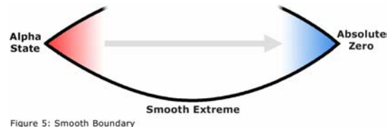
Figure 5: Smooth Boundary
