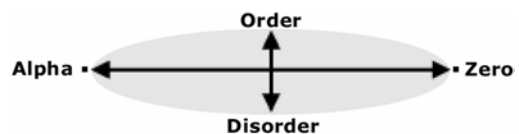
Figure 3: Admitting Zero
