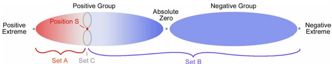
Figure 11: Probability Groups
